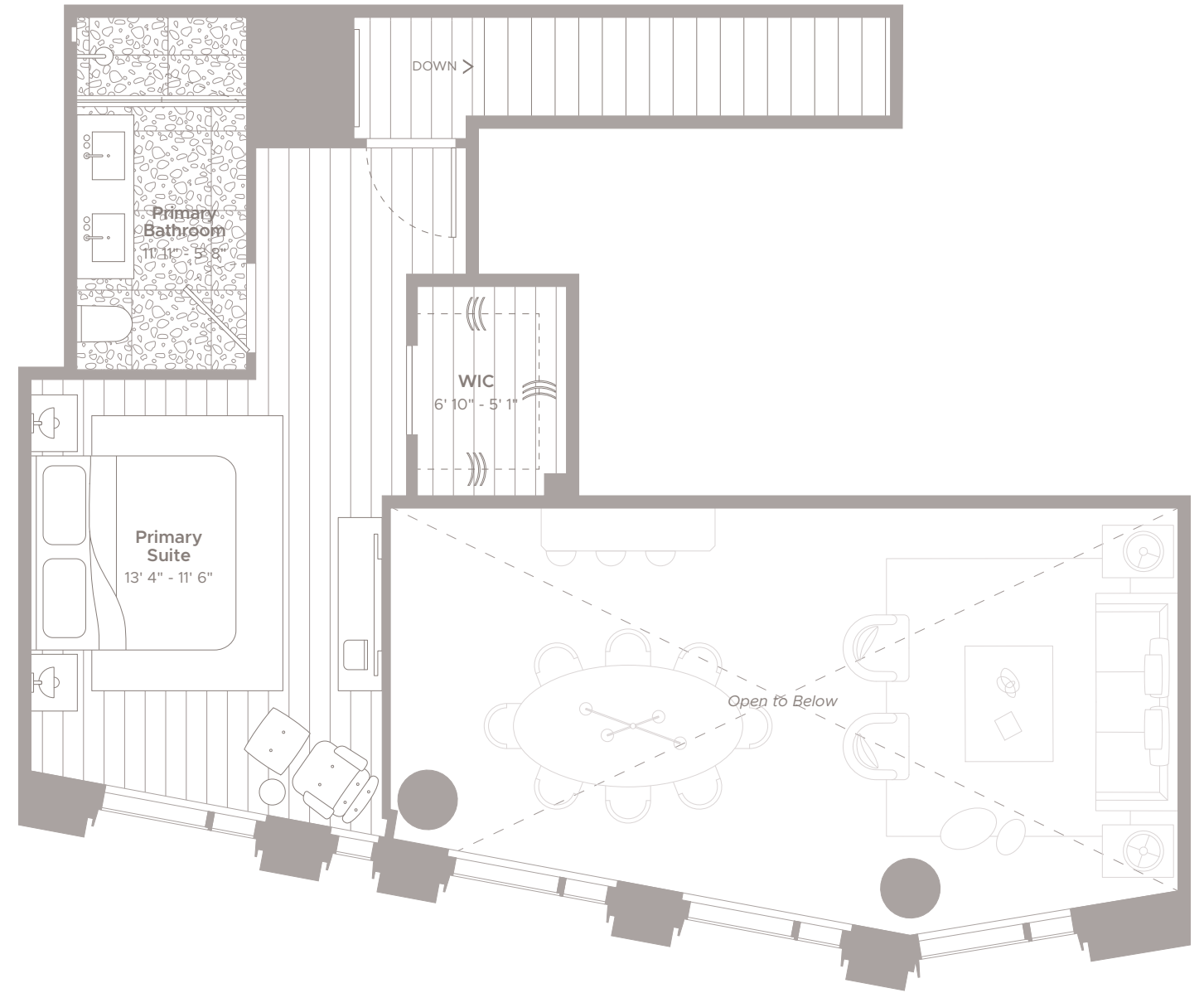
UPPER LEVEL
